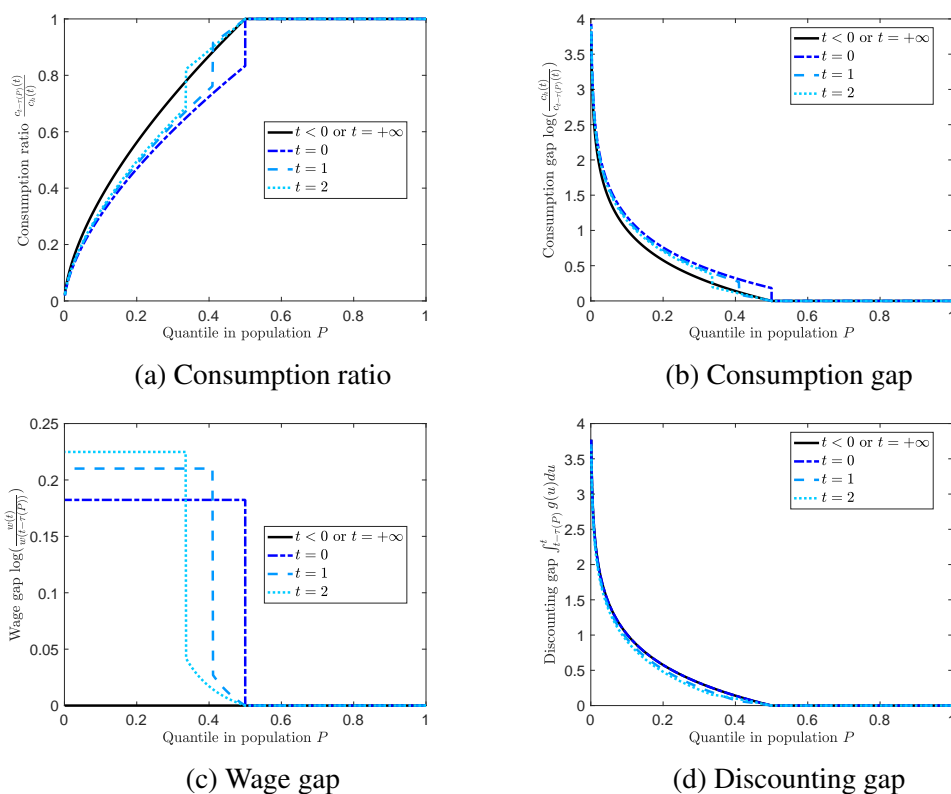
Figure B.8: Consumption inequality as a function of population quantiles, with log utility and a small permanent positive shock to A .
