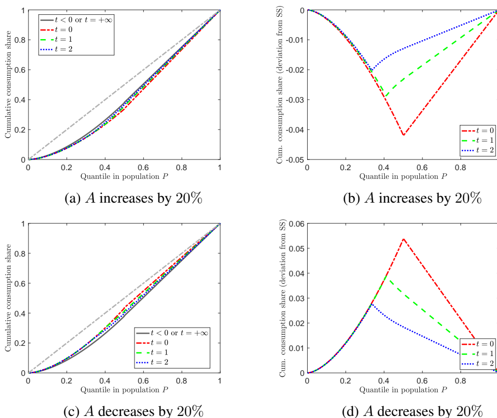
Figure 6: Evolution of the Lorenz Curve: Positive and Negative Productivity Shock.
