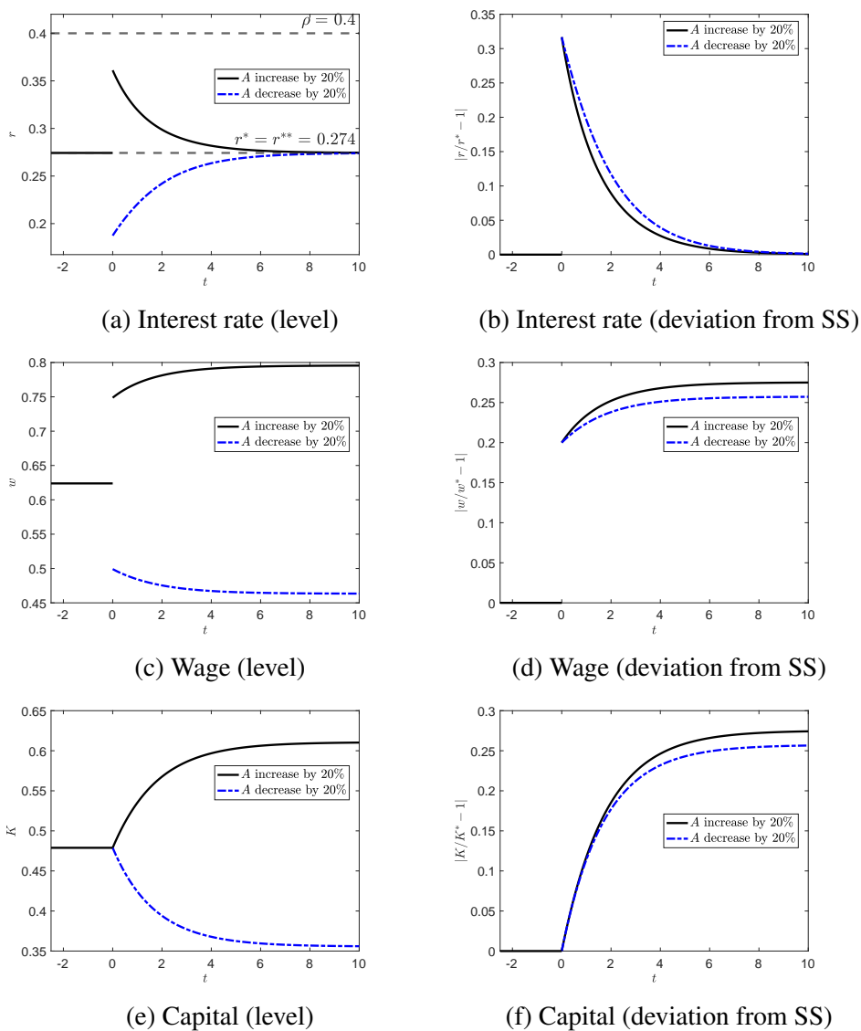
Figure 5: Transition dynamics with positive and negative permanent shocks to A .
