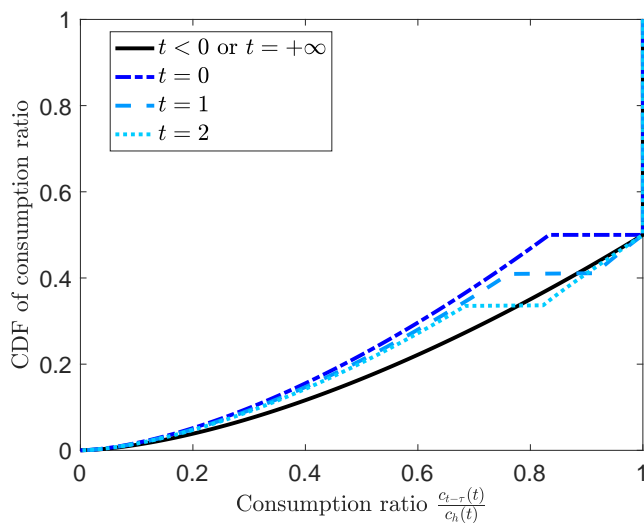
Figure B.9: CDF of consumption ratio between low income household and high income household, with log utility and a small permanent positive shock to A .
